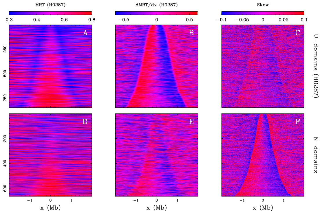
Figure S4. Same as in Supplementary Fig. S1 but for the lymphoblastoid H0287 cell line (830 replication timing U-domains).
