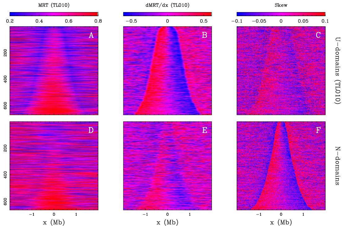
Figure S5. Same as in Supplementary Fig. S1 but for the lymphoblastoid TL010 cell line (664 replication timing U-domains).
