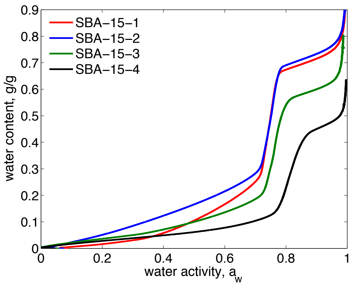
Figure S1: Water sorption isotherms of SBA-15-1 (red), SBA-15-2 (blue), SBA-15-3 (green) and SBA-15-4 (black) plotted against the water activity a_w
