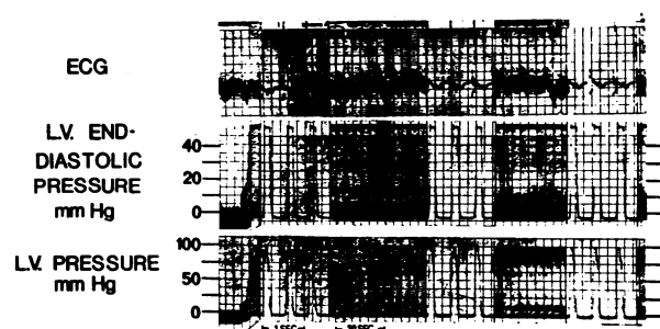
FIGURE 8 Recording of intraventricular electrocardiogram, left ventricular pressure (high gain), and left ventricular pressure when coronary bed is near maximally dilated by administration of papaverine (4.6 mg/min). Note virtually no change in S-T segment and T wave pattern (in contrast with Fig. 8) as well as minimal change in end-diastolic pressure after systolic plateau is reached.
