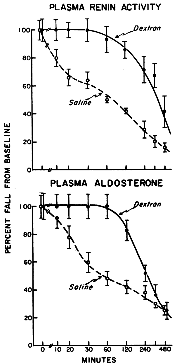
FIGURE 2 Comparison of the rate of response of PRA and aldosterone to saline and dextran infusions. Results are expressed as the mean \pm SEM% fall from the base line plotted against time on a log scale.
