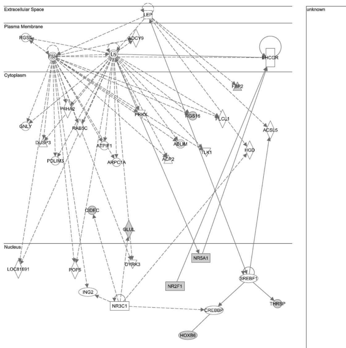
Supplementary Fig. 2 The top 3 # network significantly differentially expressed genes involved in. Solid line represents direct interaction and dash line represents indirect interaction
