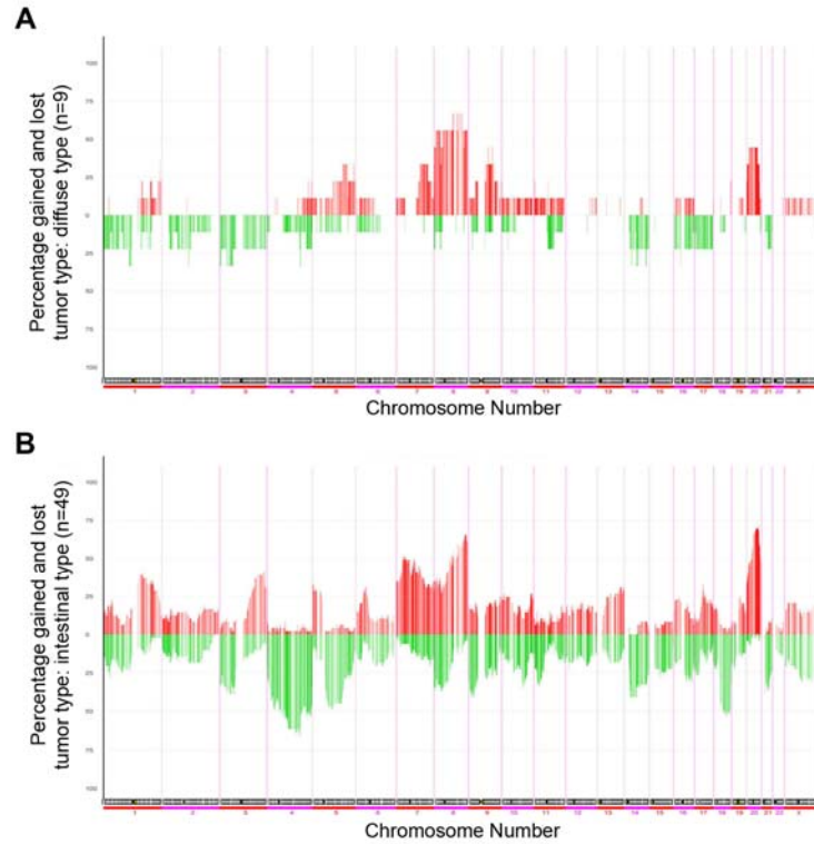
Figure S5. DNA copy number variations in gastric cancer samples with different tumor type. Data presented are ordered by chromosomal map position of the clones. Lower green bars represent losses or deletions, and the upper red bars represent gains or amplifications. (A) Tumor type: diffuse type. (B) Tumor type: intestinal type.
