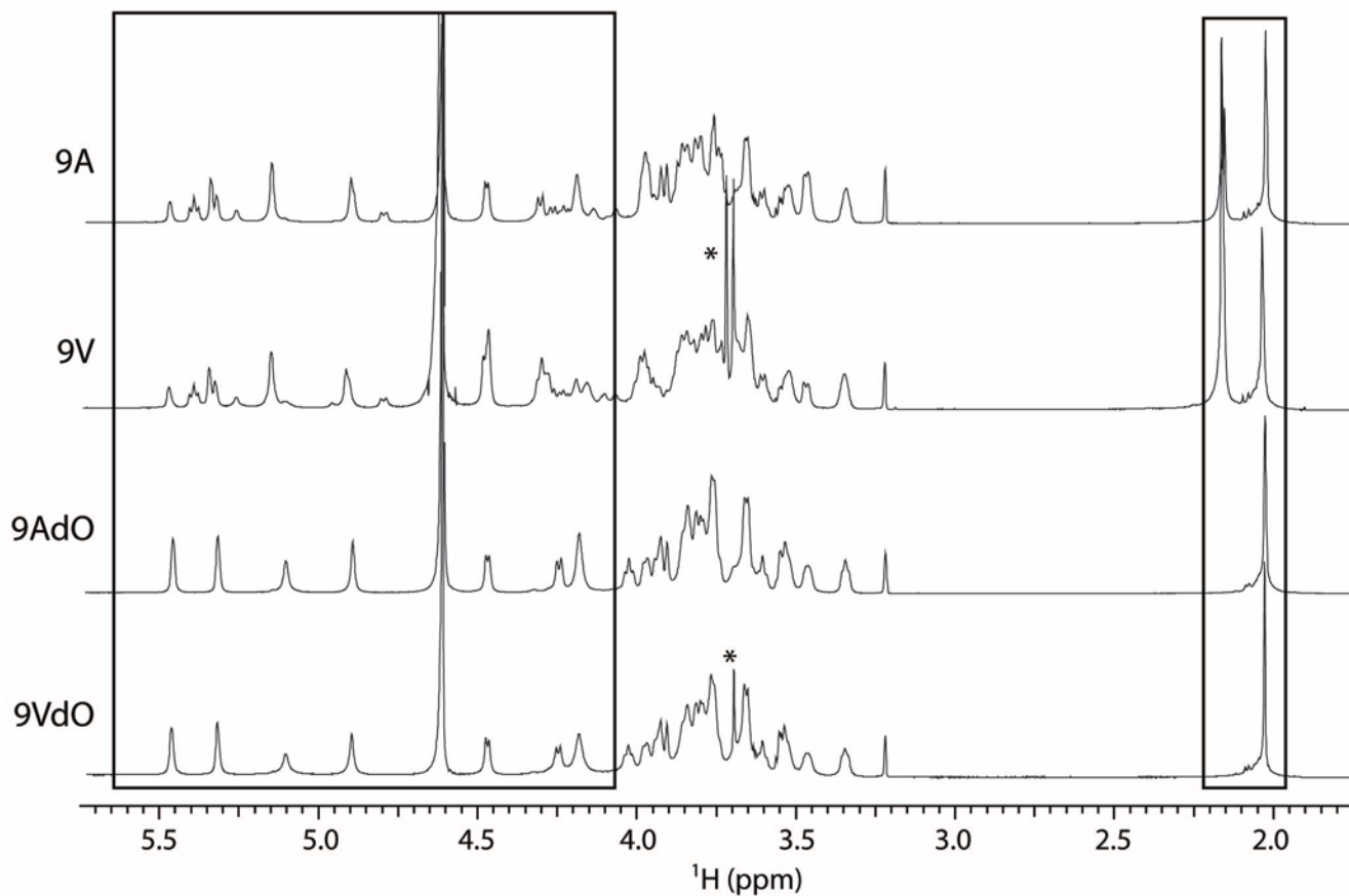
Figure S1. ^1\text{H} NMR spectra of native and de-O-acetylated (dO) 9V and 9A PS. Boxed regions are represented in figure 2A and 2B. Asterisks denote signals resulting from trace amounts of Tris.
