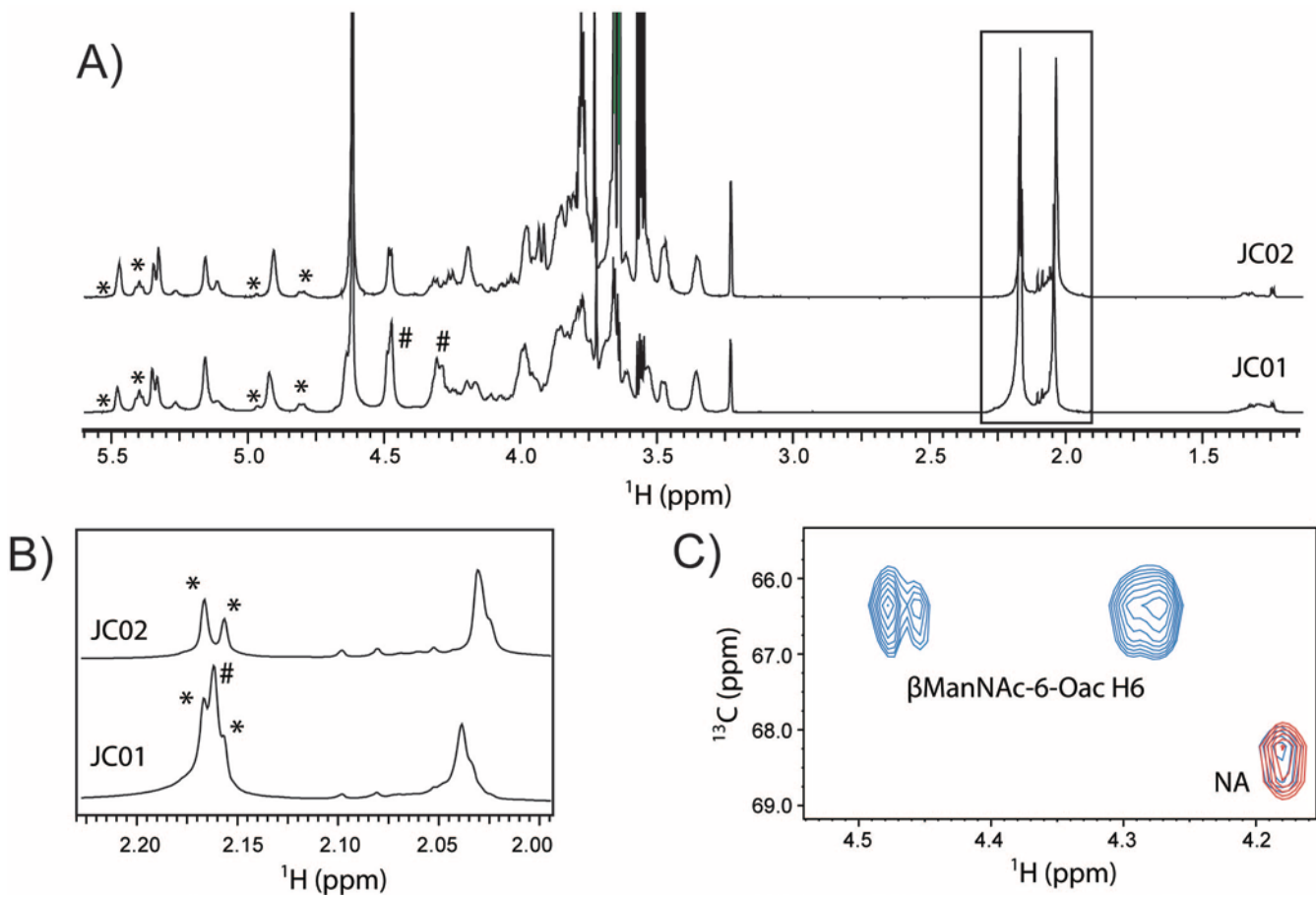
Figure S3. NMR spectra of JC01 (9V) and JC02 (9A) capsule PS. A) ^1\text{H} NMR spectra of JC01 and JC02. The area highlighted by the rectangle is enlarged in B. Asterisks in A and B denote signals that are associated with O-acetylation in both JC01 and JC02, while pound signs denote O-acetylation-associated signals present only in JC01. C) An overlay of the ^1\text{H} - ^{13}\text{C} HMQC spectra of JC01 (blue) and JC02 (red). NA, not assigned.
