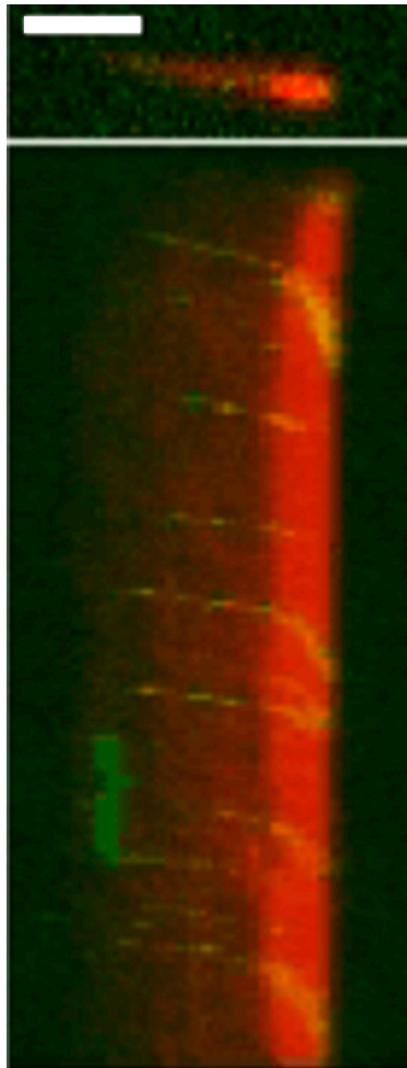
Movie S1. Formation of a traffic jam of Kip3 motors on a microtubule.
