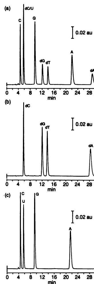
Figure 2. Reverse phase HPLC chromatograms of nucleoside mixtures. A total of 50 µg of nucleoside monophosphates were dephosphorylated with calf intestinal alkaline phosphatase prior to injection onto an Econosphere C8 reverse phase column. Elution was isocratic, with methanol-83.3 mM triethylammonium phosphate, pH 6.0 (4:96 v/v), a flow rate of 1.0 ml/min, and detection at 268 nm at 0.2 absorbance units full scale (aufs). (a) Total nucleotide pool from M. methylotrophus cellular lysate, prior to boronate affinity chromatography. (b) Deoxyribonucleotides, which do not bind to the boronate column. (c) Bound ribonucleotides, which are eluted from the boronate column.
