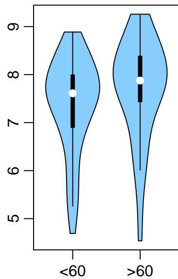
miR-218-2-3p
