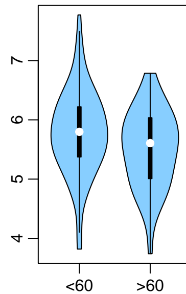
miR-181a-2-3p
