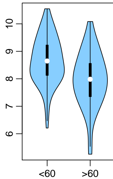
miR-215
