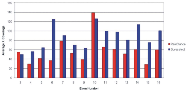
Exon coverage for LARGE
