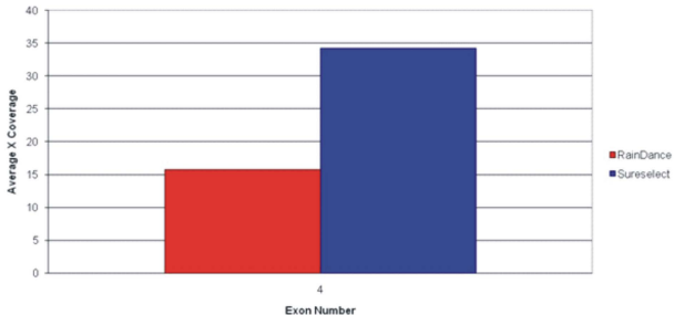
Exon coverage for FKRP
