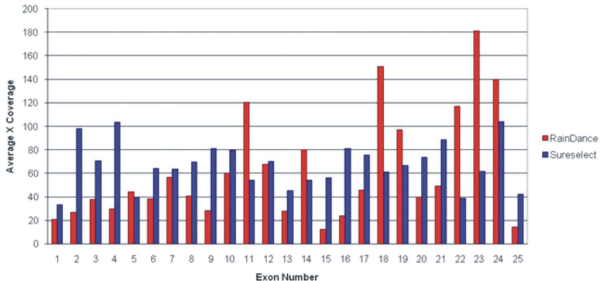
Exon coverage for ITGA7
