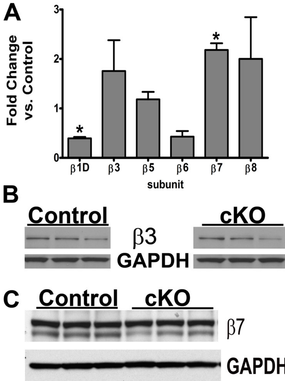
Supplemental Figure S1– Evaluation of \beta integrin transcripts and protein in cardiac myocytes from control and cKO mice.
