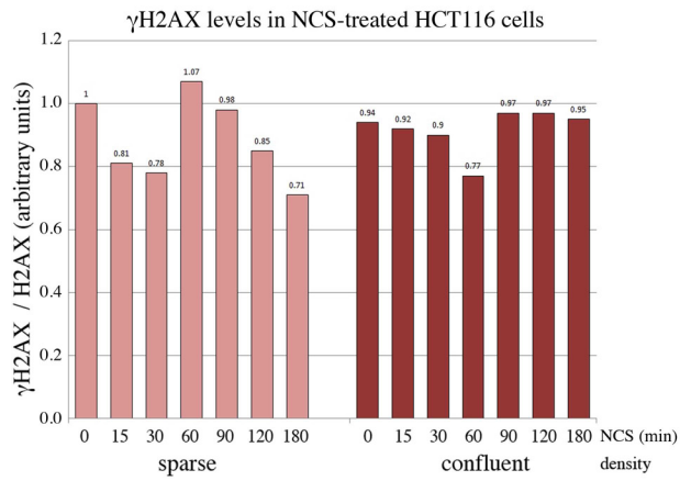
Supplementary Figure 5. Densitometric analysis was performed using the Image J software. HCT116 cells were treated with NCS as described in Figure 4B, and the levels of H2AX and \gamma H2AX were analyzed. H2AX and \gamma H2AX levels were normalized to Actin and H2AX levels, respectively.
