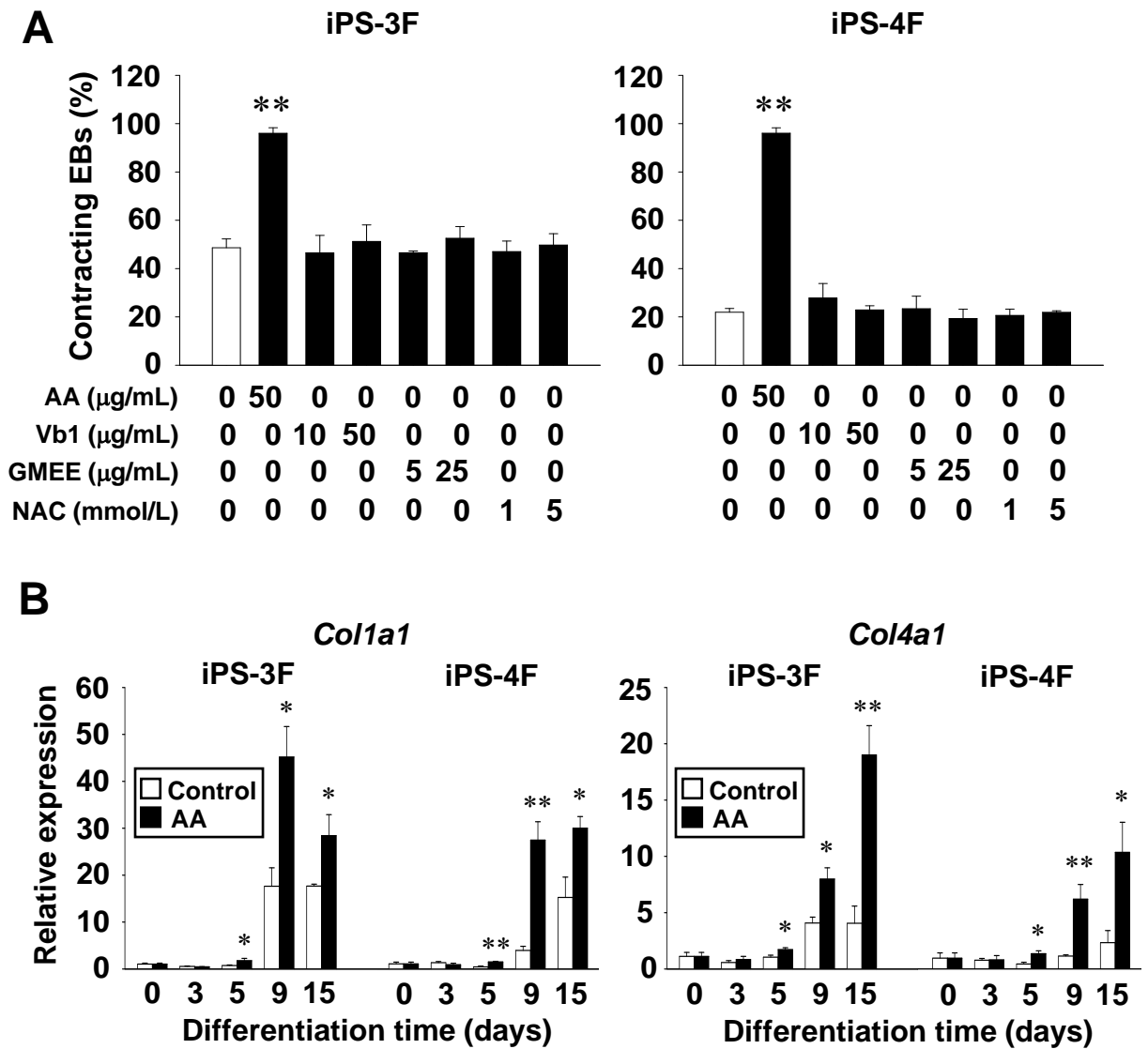
Supplementary Figure 6 AA-promoted cardiogenesis is independent of its antioxidative property. A, Antioxidants including vitamin B1 (Vb1), reduced glutathione (GMEE), and N-acetyl-L-cysteine (NAC) failed to mimic the role of AA in promoting cardiomyocyte differentiation. B, Quantitative RT-PCR analysis of the relative expression of collagen genes Col1a1 and Col4a1 . Data are collected from three experiments and expressed as means \pm SEM. * P < 0.05 , ** P < 0.01 vs. control.
