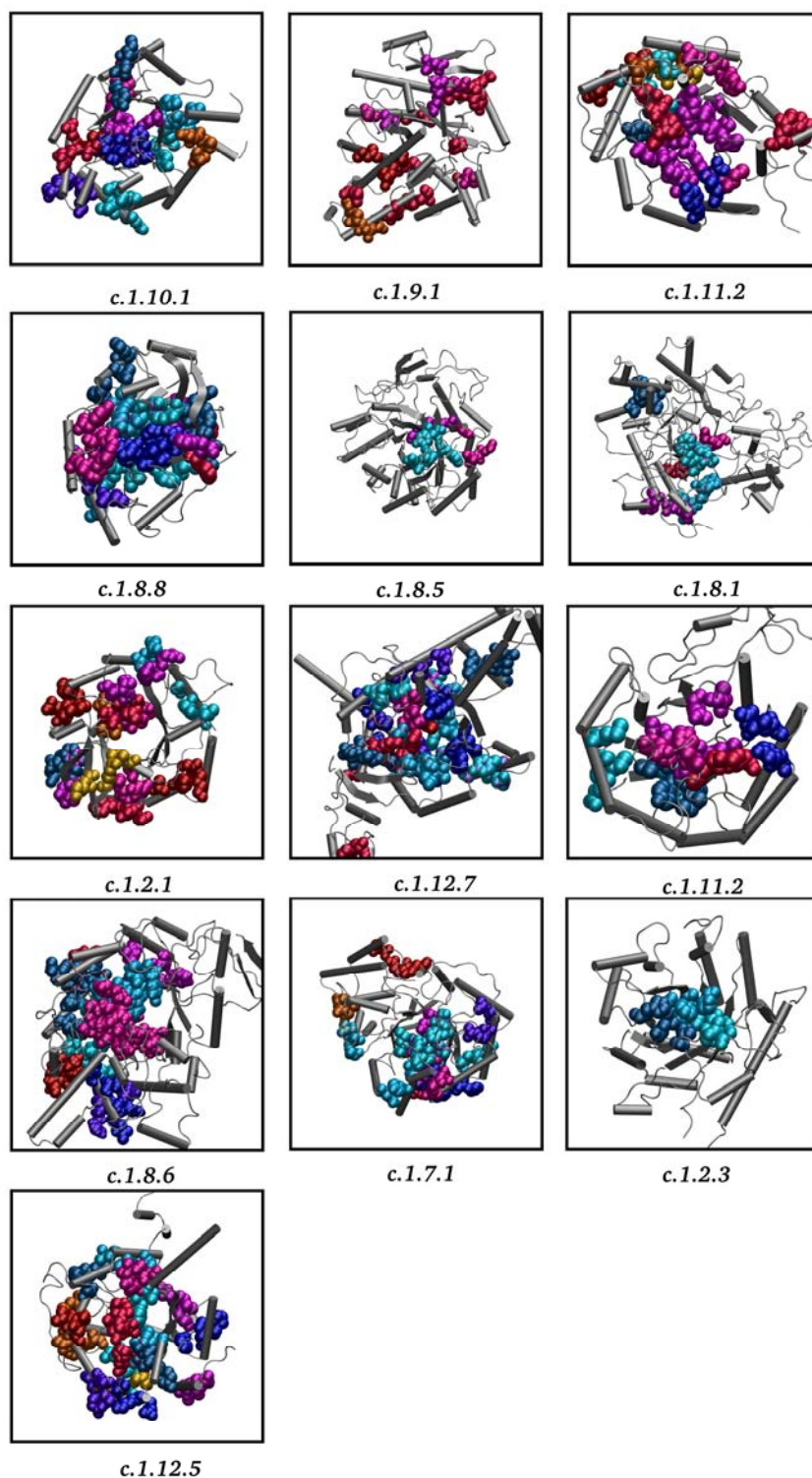
Figure S5 - Family specific clusters from the f -PENs for selected families of the TIM fold.
