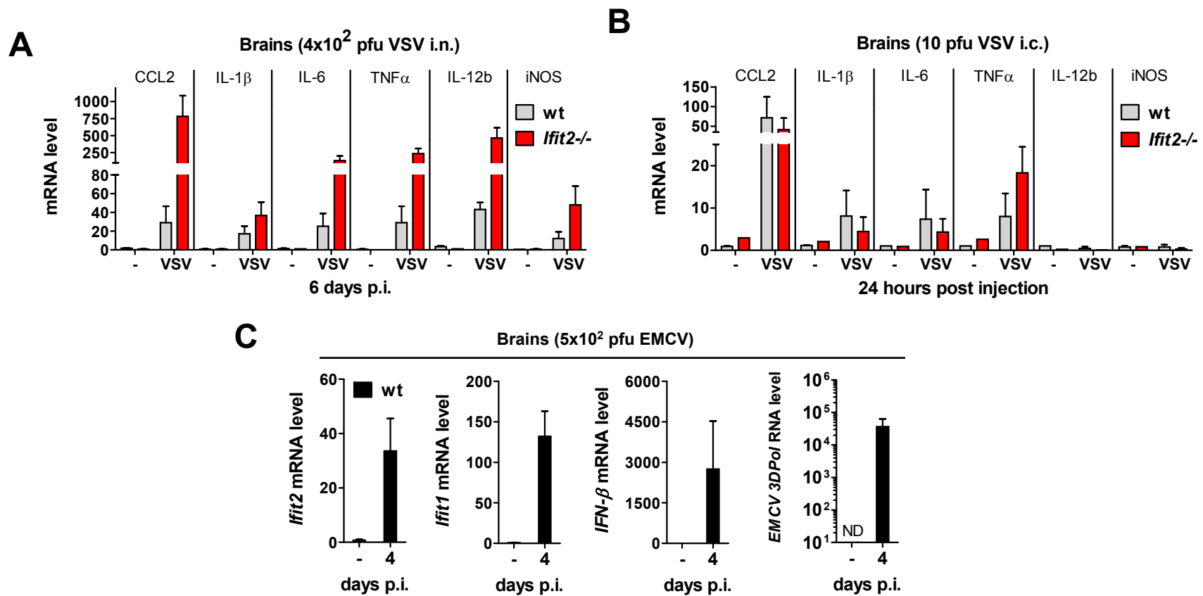
Figure S3. Gene induction in brains after VSV or EMCV infections. A , mRNA levels of select genes in brains (without OBs) of uninfected or intranasally VSV-infected wt and Ifit2 -/- mice at 6 d.p.i., plotted as mean+SD; n=3 mice per infected group; infection was intranasal with 4 \times 10^2 pfu of VSV B , mRNA levels of select genes in brains (without OBs) of uninfected or intracranially VSV-infected wt and Ifit2 -/- mice at 24 h post injection, plotted as mean+SD; n=4 mice per infected group; infection was intracranial injection with 10 pfu of VSV. C , Ifit2 , Ifit1 , IFN- \beta and EMCV RNA levels in brains 4 days after EMCV infection ( 5 \times 10^2 pfu, n=3 mice per infected group).
