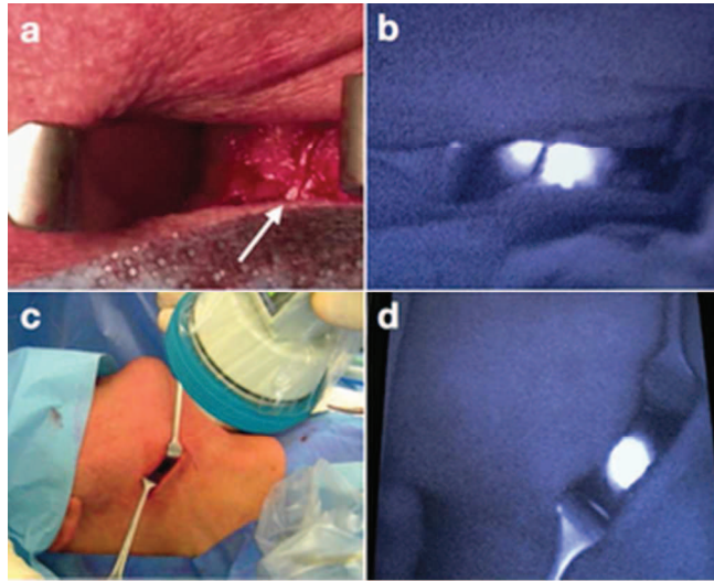
FIG. S1 Visualization of the fluorescent component of the hybrid tracer in sentinel nodes in the neck region. a, b The near-infrared light camera reveals the sentinel node underneath a thin layer of muscle and covered by a small vein (arrow). c, d Another non-blue sentinel node is clearly visualized using the fluorescence camera 27x22mm (300 x 300 DPI)
