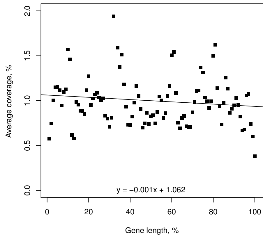
RNA-seq, SOLiD
