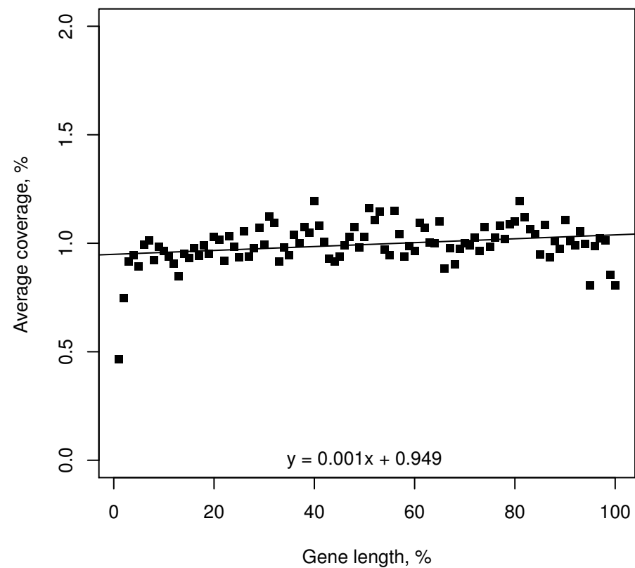
Genomic, SOLiD
