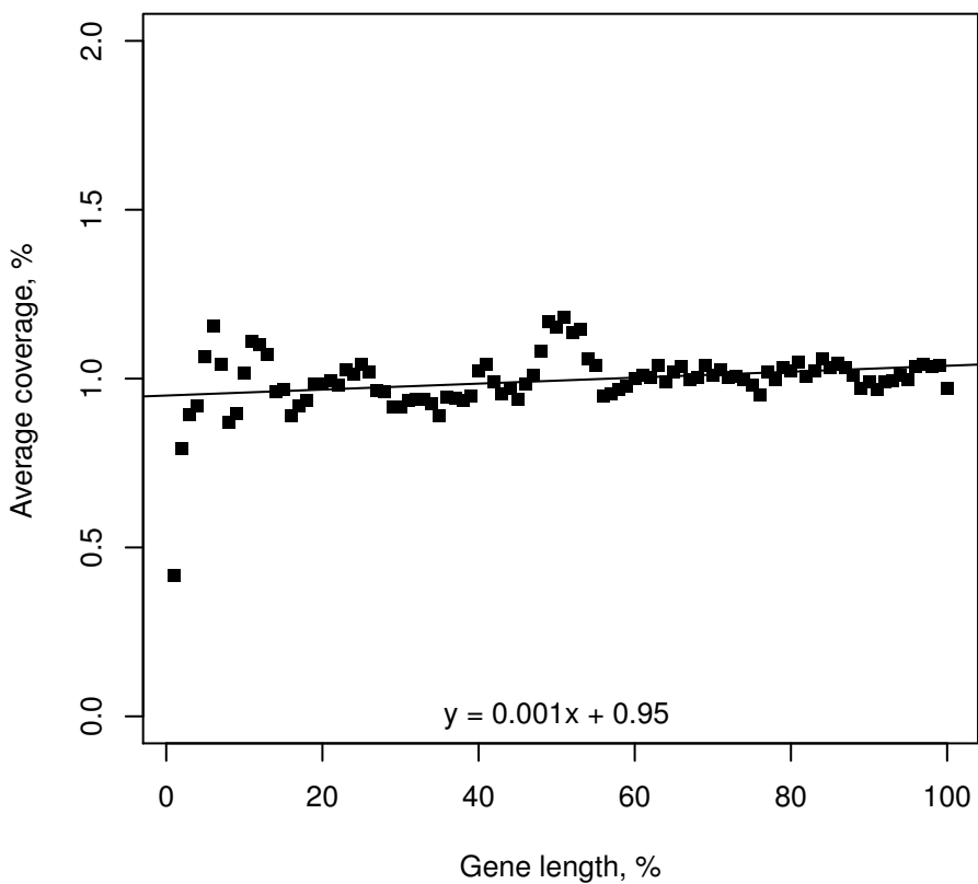
Genomic, Illumina
