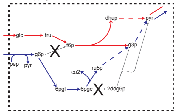
(C) Role of Hexokinase in iJR Dominant Ethanol Production. Deletions: edd , 6-phosphogluconate dehydratase pgi , glucose-6-phosphate isomerase
