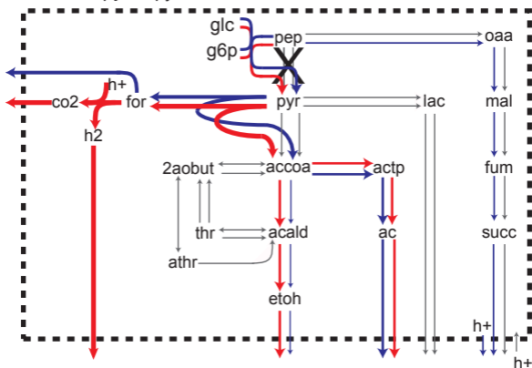
(B) Role of Hydrogen Transport in iJR Dominant Ethanol Production. Deletions: atpB , ATP synthase
