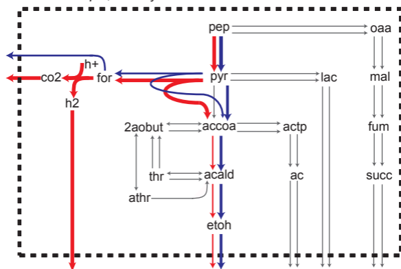
(B) Role of Hydrogen Transport in iJR Dominant Ethanol Production. Deletions: atpB , ATP synthase
