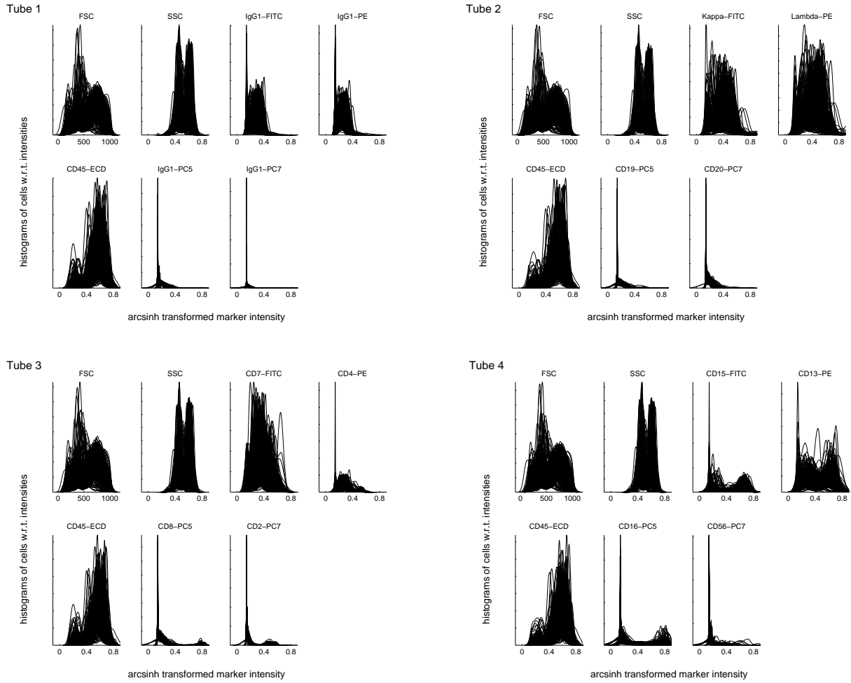
Figure S1: Distributions of marker intensities in data of tubes 1-4. Each small panel contains 359 curves, and each curve shows the distributions of the intensities of one marker in one tube for one of the 359 samples.
