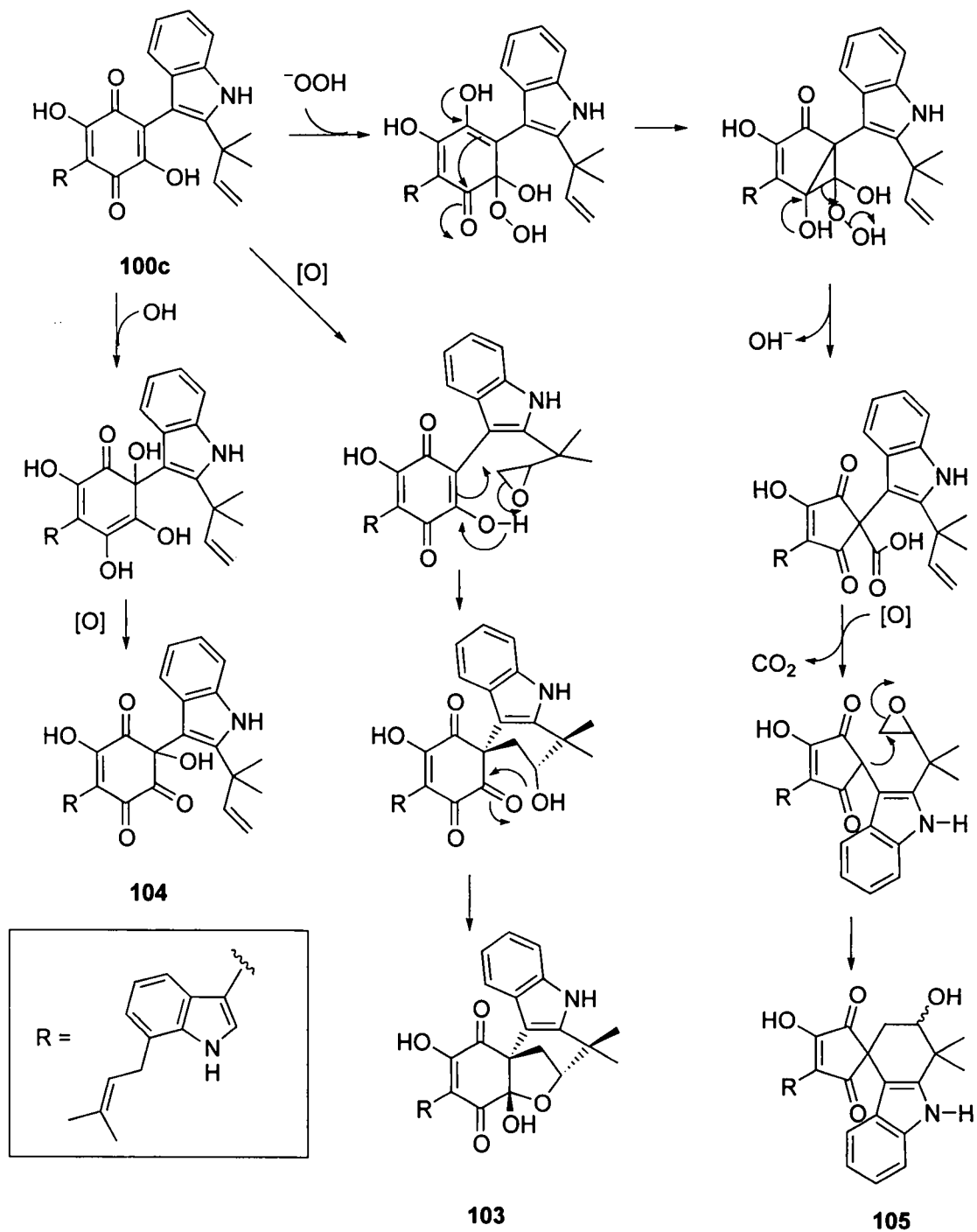
Figure S1. Possible biosynthetic pathways to Pseudomassaria metabolites 103, 104, and 105 from DMAQ-B1 (100c).
