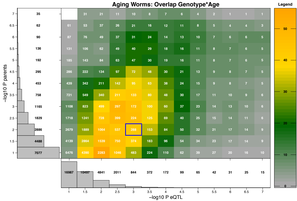
Figure S4 Number of overlapping genes between differentially expressed genes in the parental strains and with at least an eQTL at different thresholds in old worms with genotype*age interacting effect. See Figure S1 legend for details.
