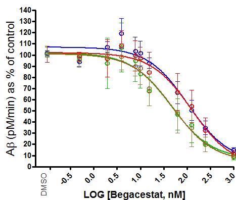
Begacestat
