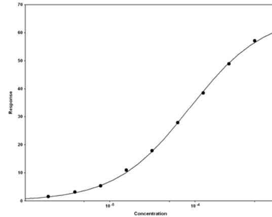
FIGURE S3. Surface plasmon resonance of C3.1 scFv binding to (a) 1 , (b) 2 , and (c) 3 at equilibrium. Representative sensograms (left panels) and fits of the response at equilibrium (right panels) from the SPR binding assays. Numbers in brackets are the standard deviation.
