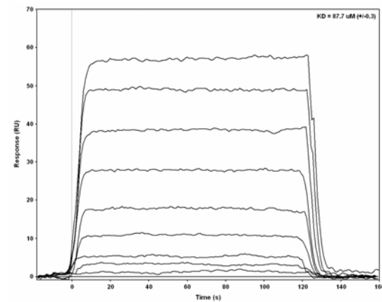
FIGURE S3. Surface plasmon resonance of C3.1 scFv binding to (a) 1 , (b) 2 , and (c) 3 at equilibrium. Representative sensograms (left panels) and fits of the response at equilibrium (right panels) from the SPR binding assays. Numbers in brackets are the standard deviation.
