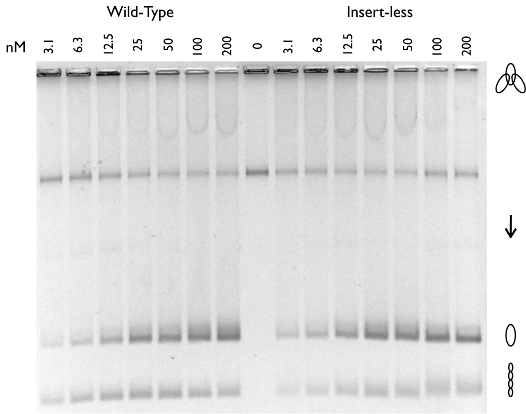
FIGURE S2. Wild-Type and Insert-less E. coli holoenzyme decatenation assay. The positions of the kinetoplast network, relaxed released circles, and supercoiled released circles are labeled with cartoon representations on the right.
