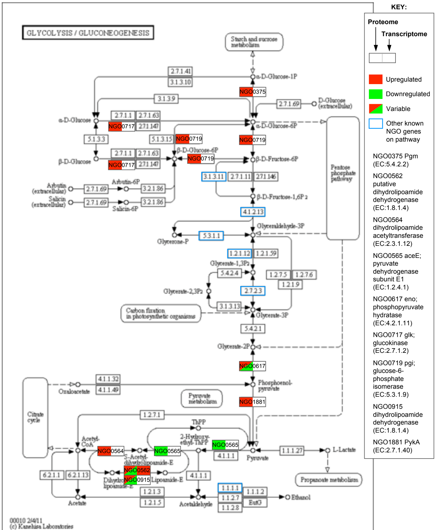
Supplementary Figure S4. KEGG pathway for glycolysis/gluconeogenesis.
