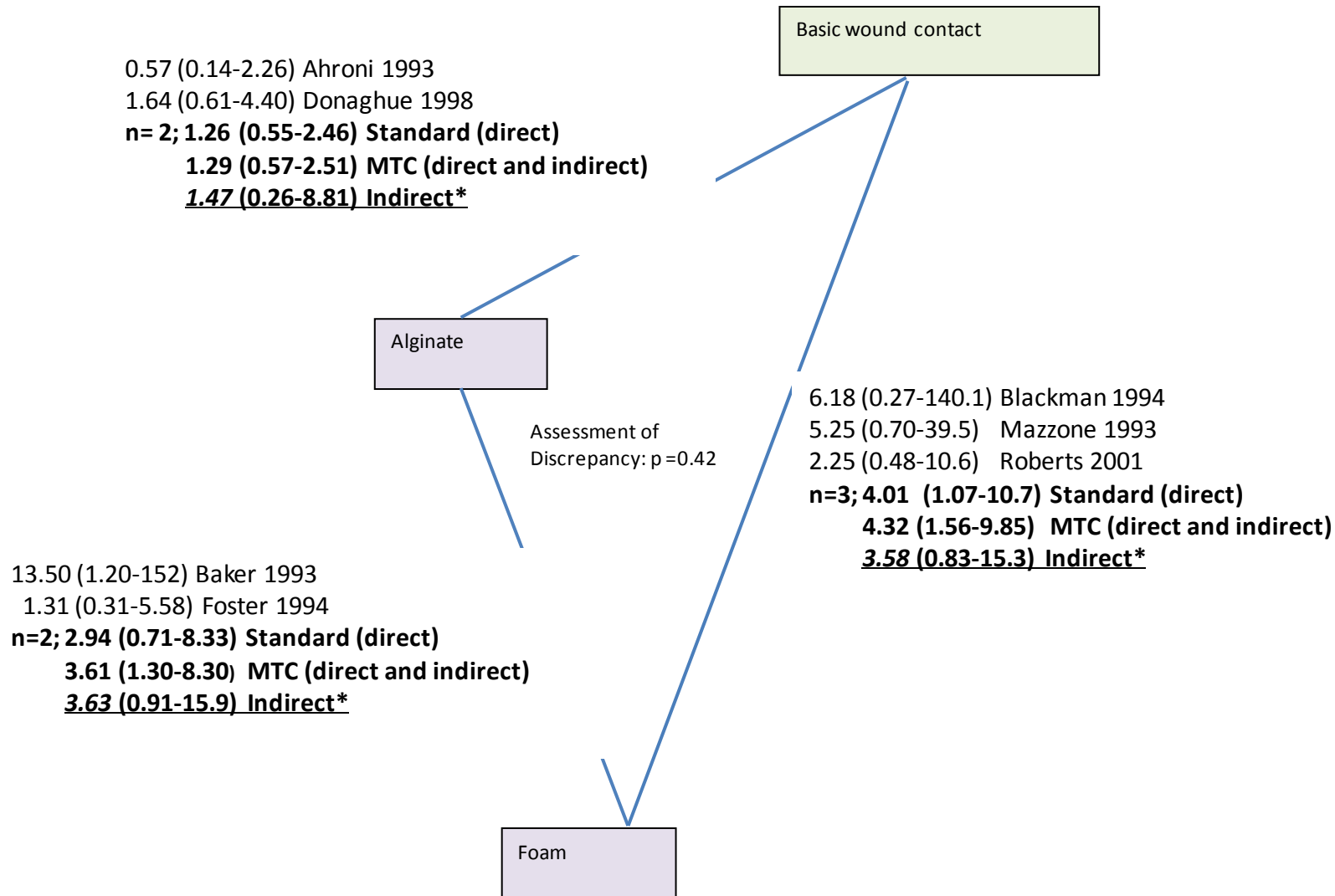
ESM Fig. 1 Assessment of inconsistencies in data loop. From top to bottom for each link: Study ORs, results from standard fixed effects meta-analysis, results from MTC, results when relative effect estimated with only indirect data (direct data removed), results of statistical analysis of direct versus indirect evidence data. * Median rather than mean values have been presented for indirect data.
