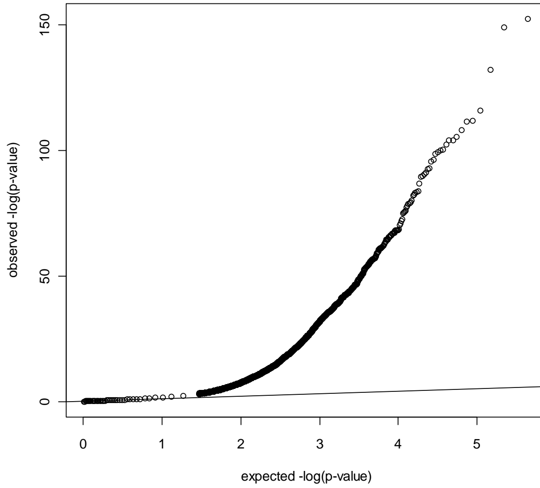
Q-Q Plot
