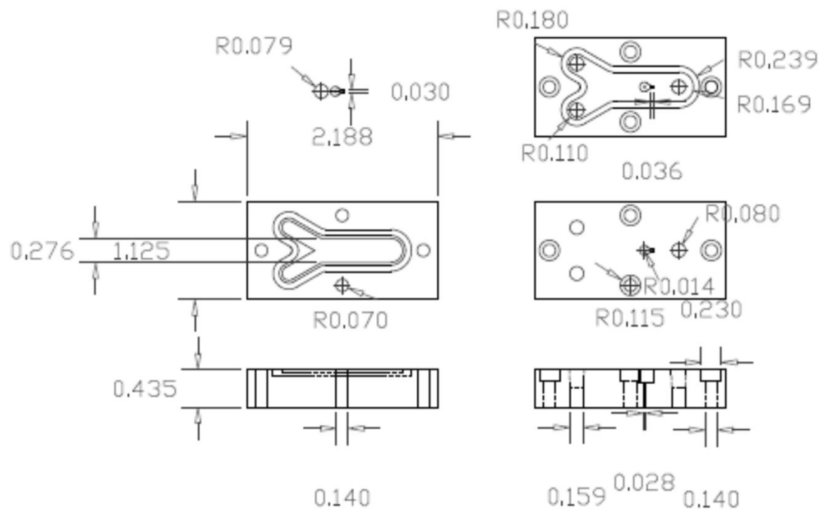
Microfluidic Flow Cell (units in inches)
