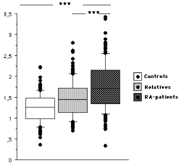
Figure 3a. CCPIgM
