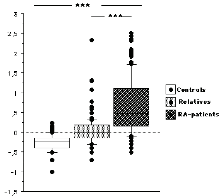
Figure 3b. CCPIgA
