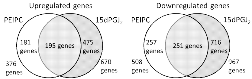
Figure S1: Venn diagram of overlap in PEIPC and 15dPGJ 2 -regulated genes in HAECs using genes up- or down-regulated by at least 1.5 fold vs. control-treated cells
