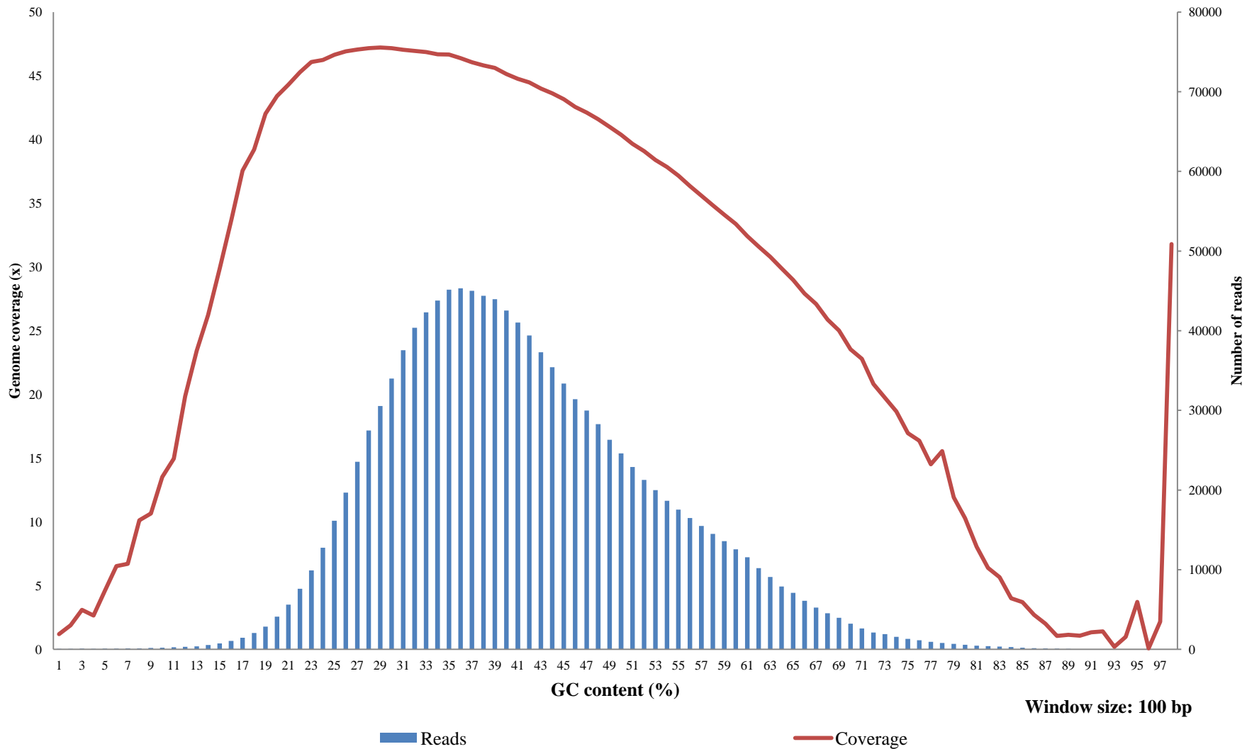
Relationship between read depth coverage and GC content throughout dog chromosome 1
