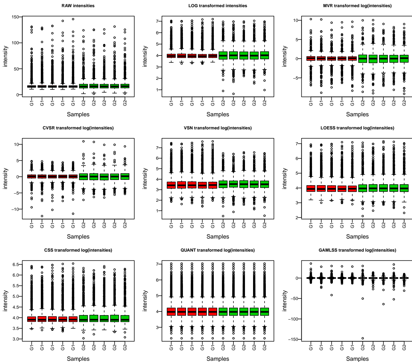
Supplementary Figure 7: Box-whisker plots of intensities by sample and group before and after transformation for the synthetic dataset. Red and green colors refer to the two sample groups. Results are shown for the synthetic dataset from model 14.
