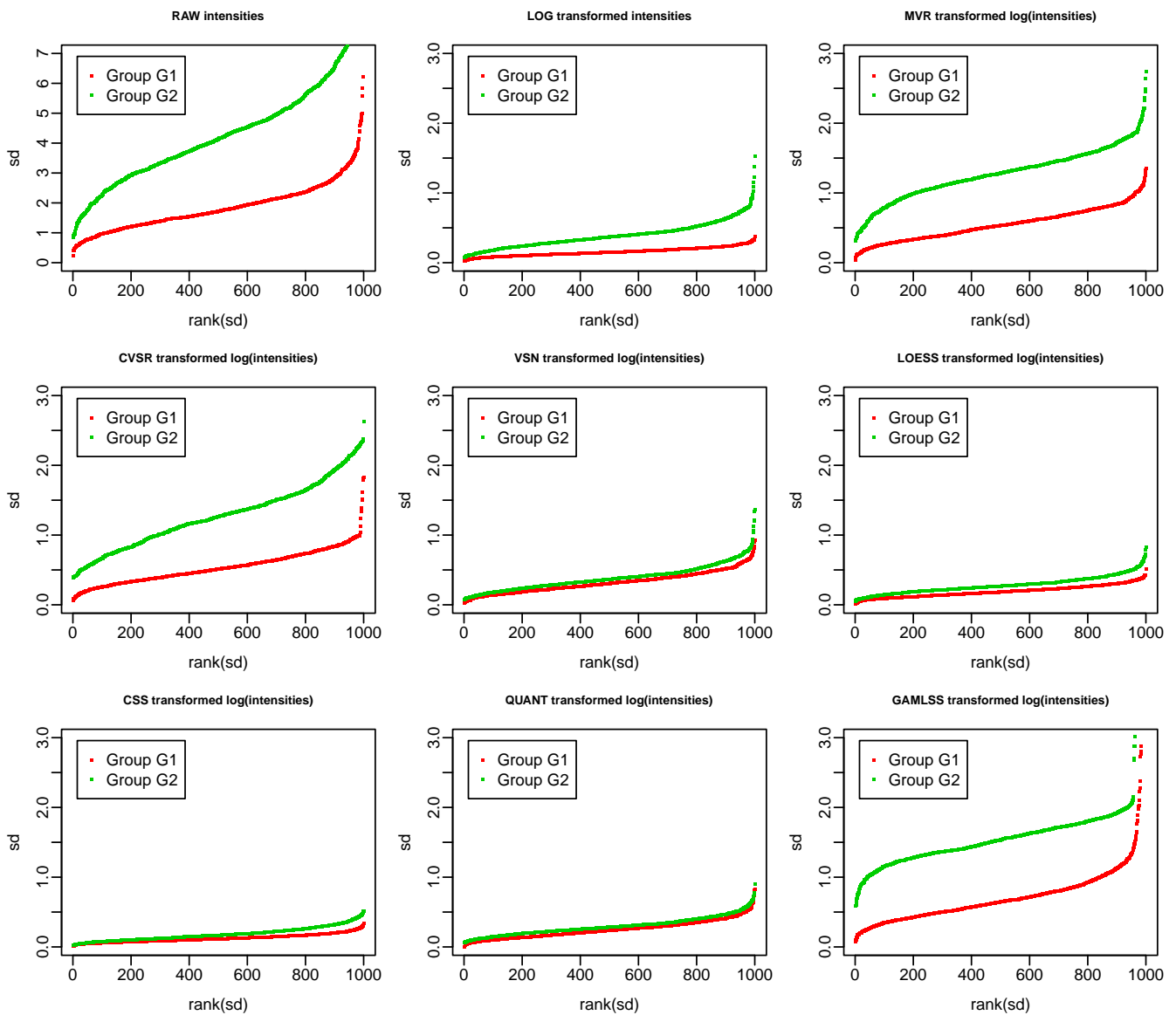
Supplementary Figure 8: Comparative sample group homoscedasticity plots for the synthetic dataset. The sample group standard deviations ( sd ), computed by group, are plotted against their ranks ( rank(sd) ) under various transformations and variance stabilization procedures. Note the difference in scale of the standard deviations in the raw data case as compared to all other transformations (on an identical scale). Results are shown for the synthetic dataset from model 14.
