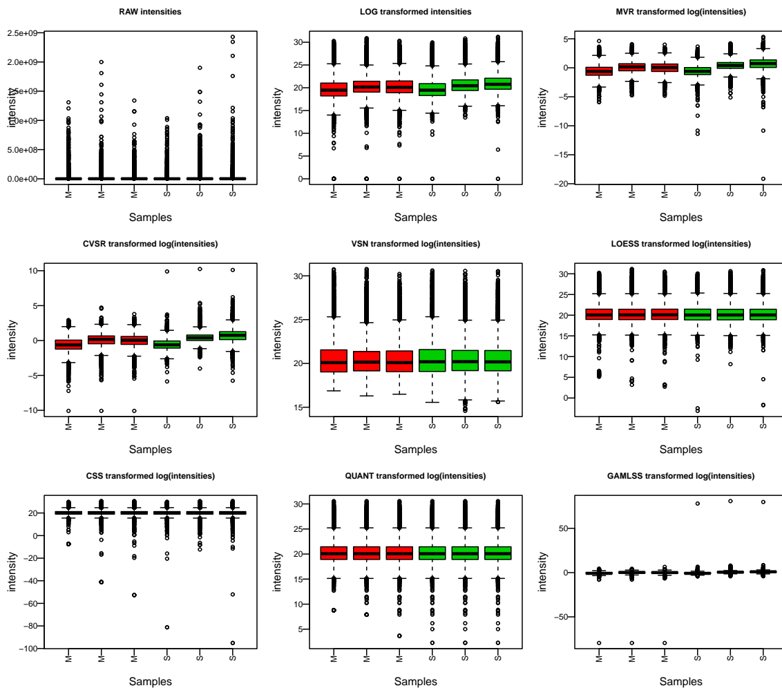
Supplementary Figure 10: Box-whisker plots of intensities by sample and group before and after transformation for the real proteomics dataset. Red and green colors refer to the two sample groups.
