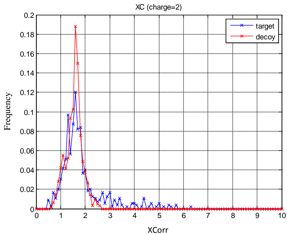
Supplemental Figure 1. Example of peptide filtering. A plot of the frequency of XCorr values at charge state 2 for the matched target and decoy soybean database entries after SEQUEST searches and applying a 5 ppm filter. An XCorr filter of 2.81 obtained an estimated FDR of 0.12%.
