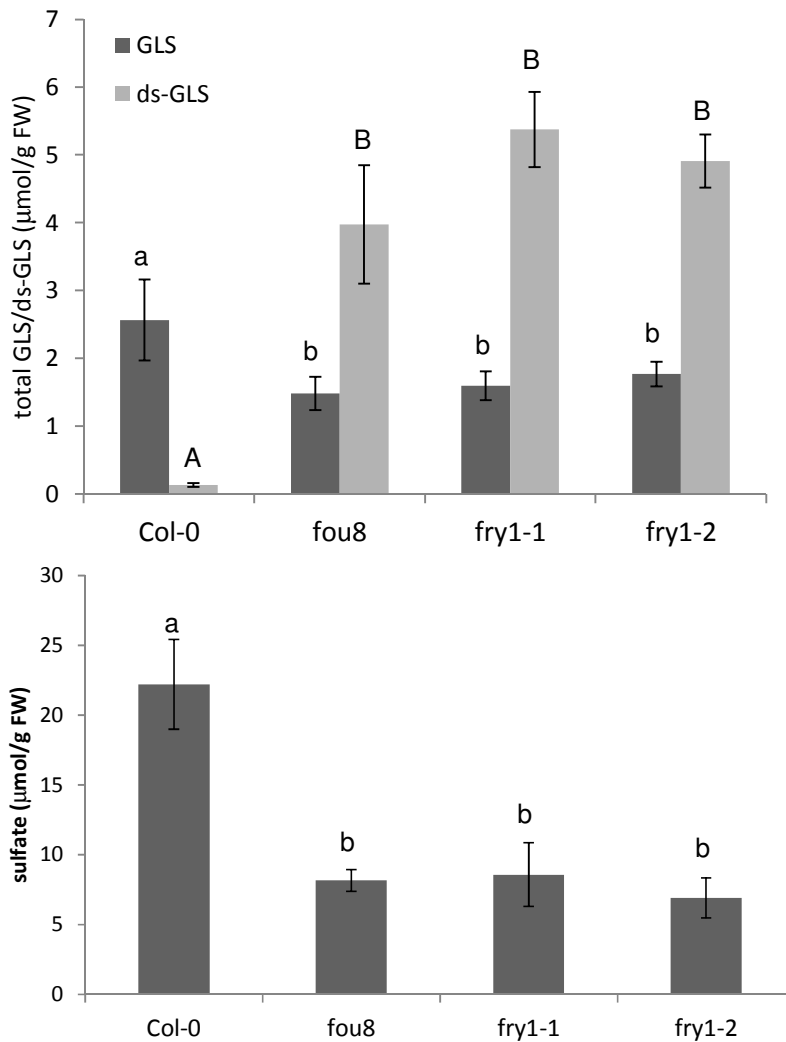
Supplemental Figure S2. Glucosinolate and sulfate accumulation in different alleles of fry1 .
