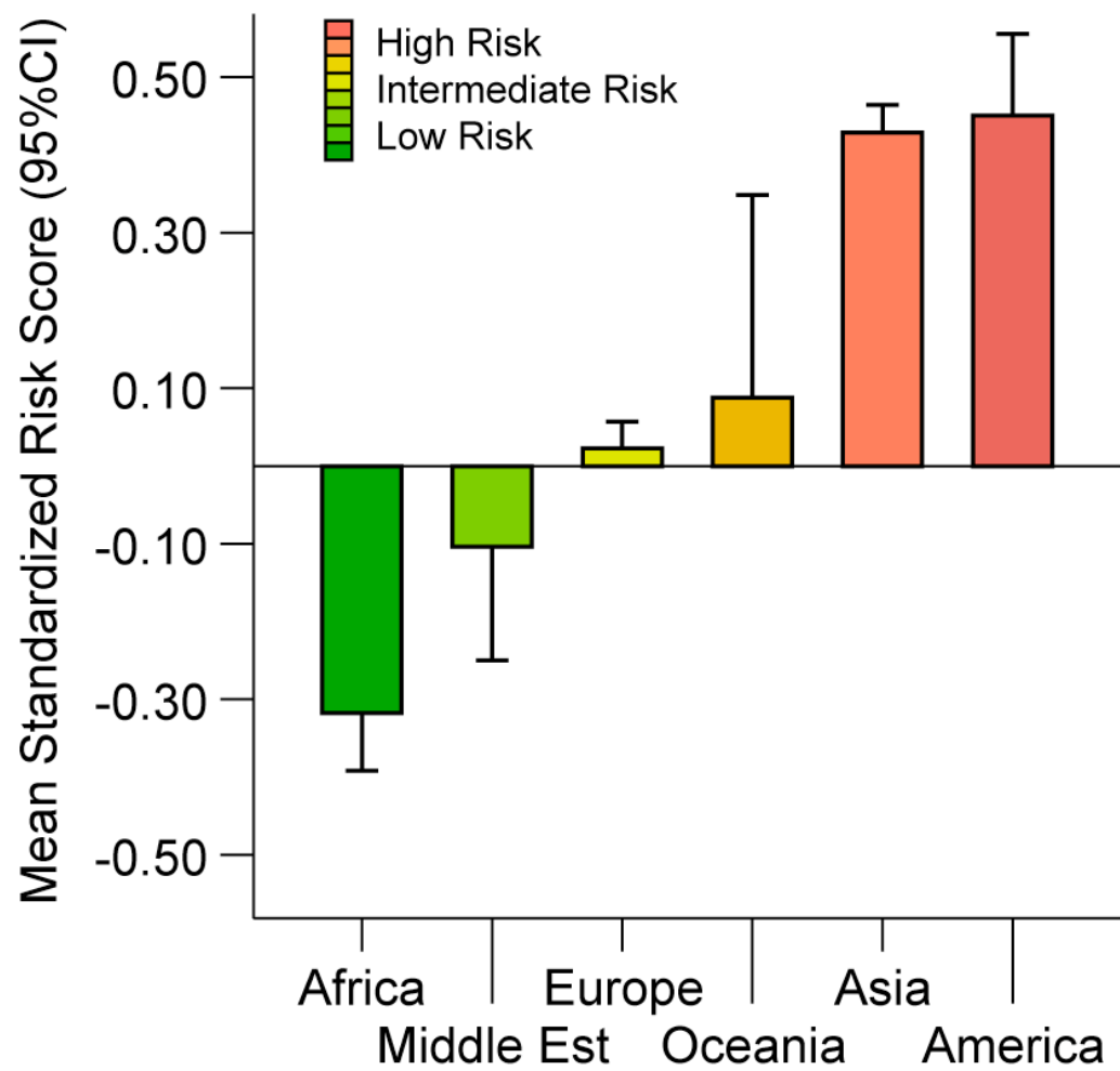
Supplemental Figure 2. Inter-continental differences in the genetic risk score based on 85 worldwide populations used for geospatial analysis.
