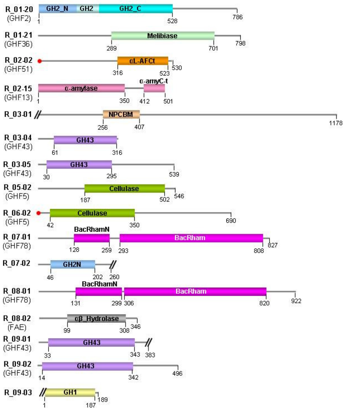
Figure S4 Domain organisation of the rumen hydrolases identified in the present work, according to sequence using the Pfam database. The signal peptides predicted using the SignalP server are indicated with a red dot at the N-terminal site.
