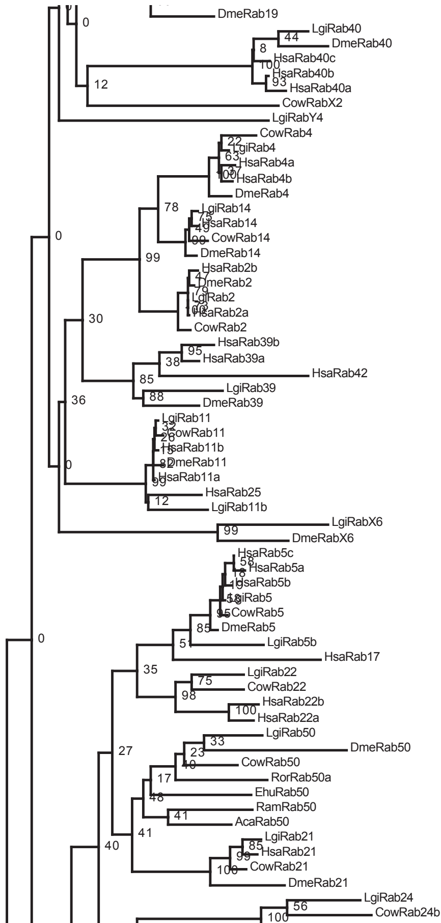
Elias et. al. Figure S13: PhyML_page2
