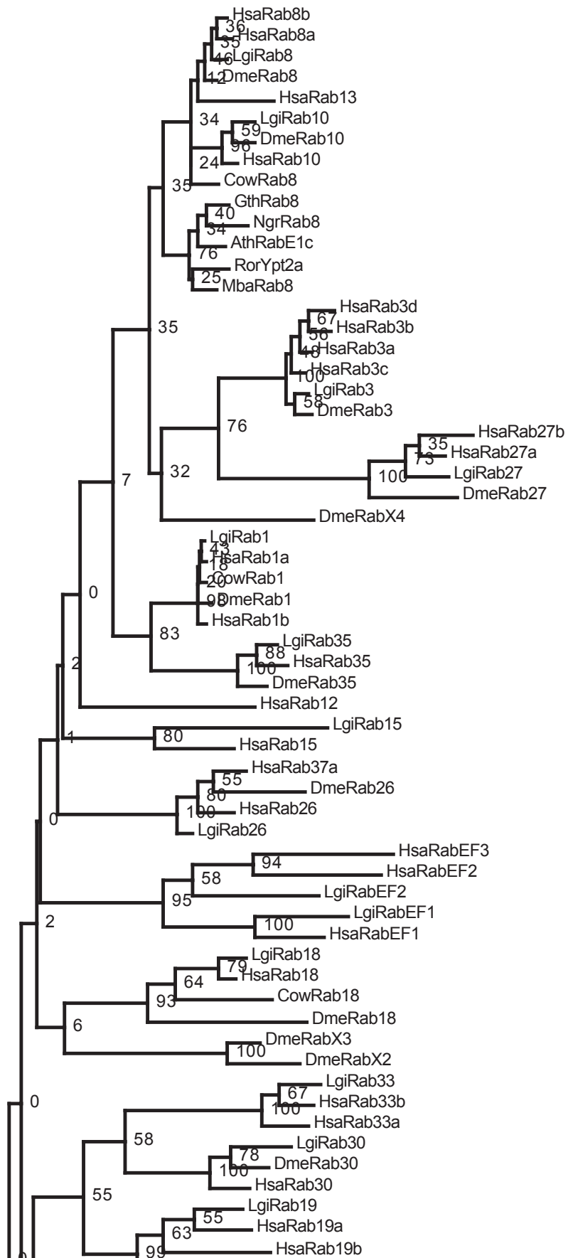
Elias et. al. Figure S13: PhyML_page1
