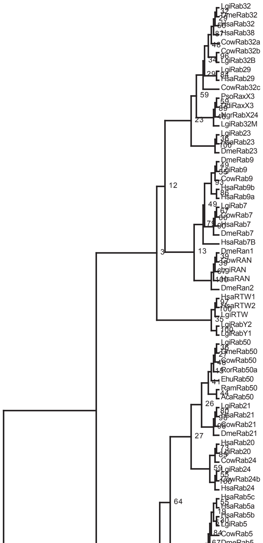
Elias et. al. Figure S13: RAXML_page1
