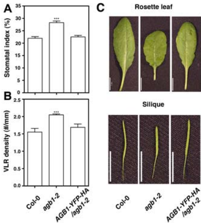
Figure S1. Phenotypic analysis on the 35S:AGB1-YFP-HA/agb1-2 complementation line.
