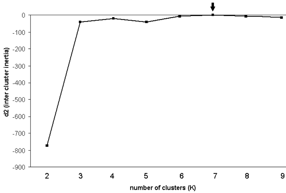
Fig. S1 Second derivative of the inter cluster inertia of each number of groups (K) as estimated by the nonhierarchical K-means clustering.
