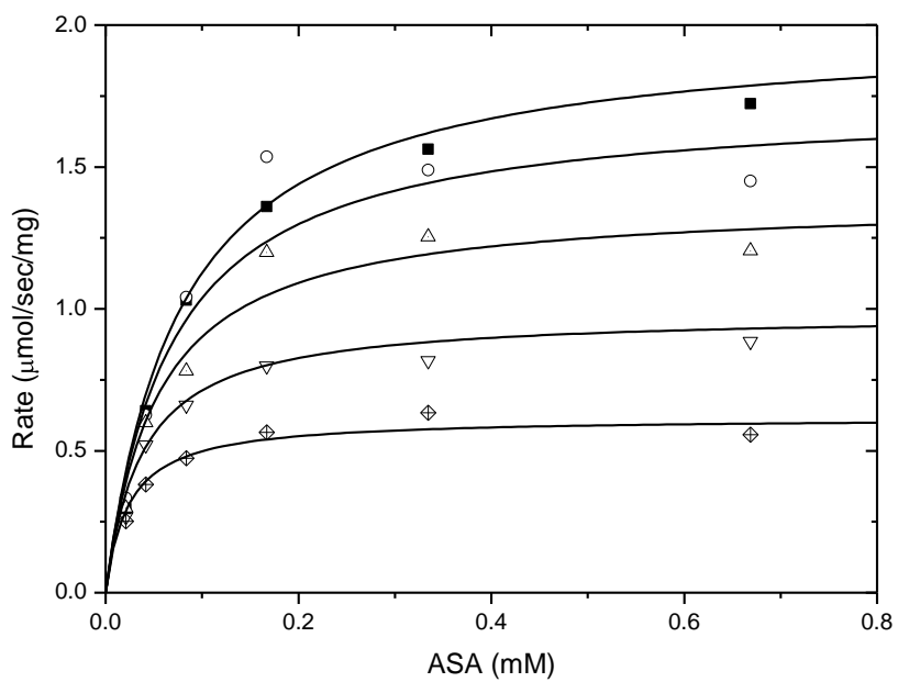
Fig S2: Kinetics of At-DHDPS2 . Assays were carried out at varying concentrations of (S)-lysine (top panel), or varying concentrations of ASA and pyruvate (bottom panel).
