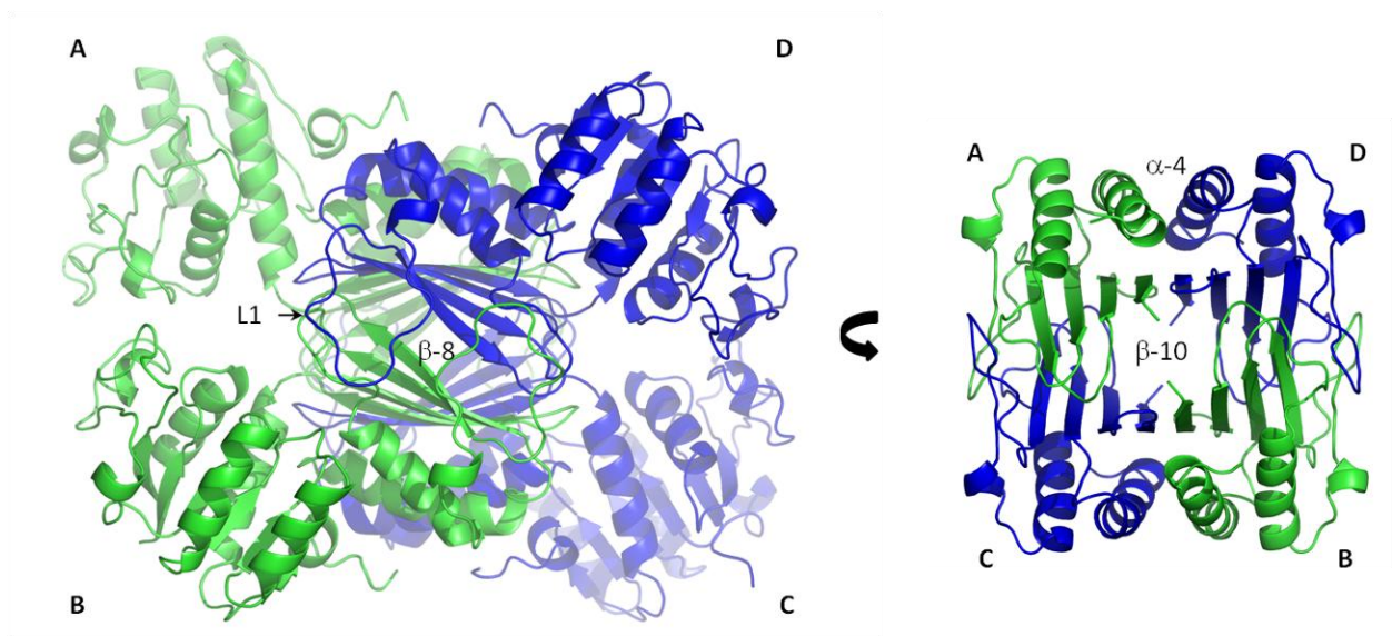
Figure S4: Structure of bacterial DHDPR. The structure of Ec -DHDPR (pdb: 1arz), showing the interface between \beta -8 and loop 1 (left panel) and the alternate interface involving \beta -10 and helix-4 (right panel, only the C-terminal domain shown).
