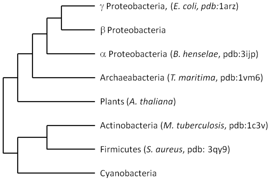
Figure S8: Representative phylogenetic tree of DapB orthologues based on Hudson, 2005 [5].
