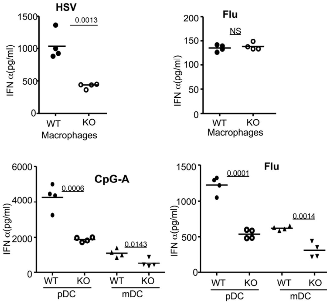
Supplementary information, Figure S2 Responses of TLR9 and TLR7/8 pathway in macrophages and in mDC. The type 1 interferferon production was measured from BM-derived macrophages and monocyte-derived dendritic cells (mDC) as well as from pDC of WT and KO mice stimulated by CpG-A, Flu and HSV. These data are representative of two independent experiments performed in duplicates.
